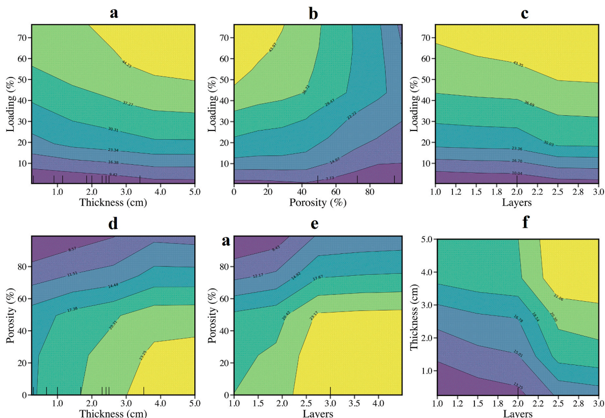
Fig. 4. Bivariate partial dependence plots of the features.
